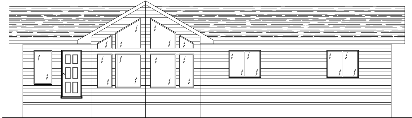
FRONT ELEVATION
